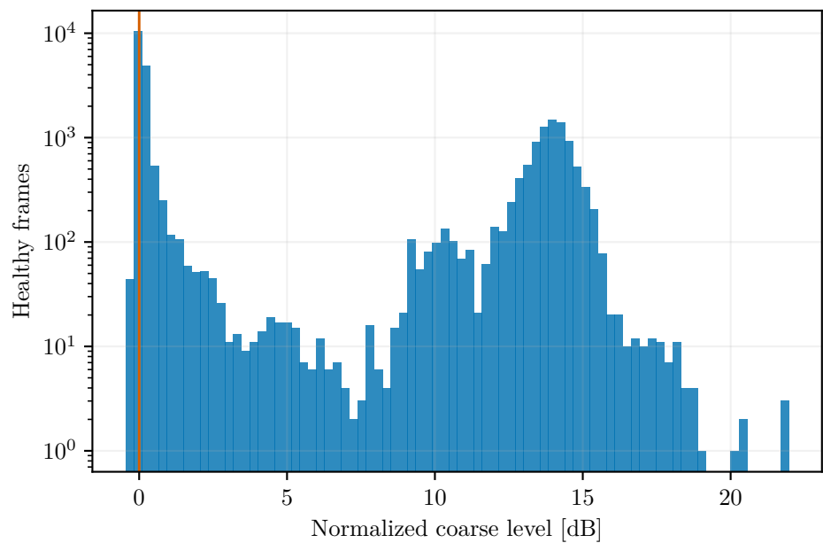
Channel 26 (frequency ID 660): health-filtered scalar distributions N=26,348; stored coarse mask rate 95.32%
