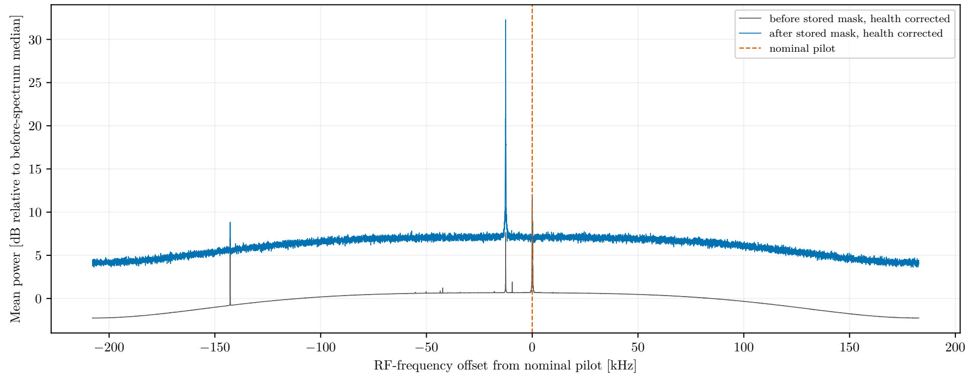
Channel 28 (frequency ID 629): relative time-averaged spectra exact v1 DC subtraction: 13 before, 13 after
