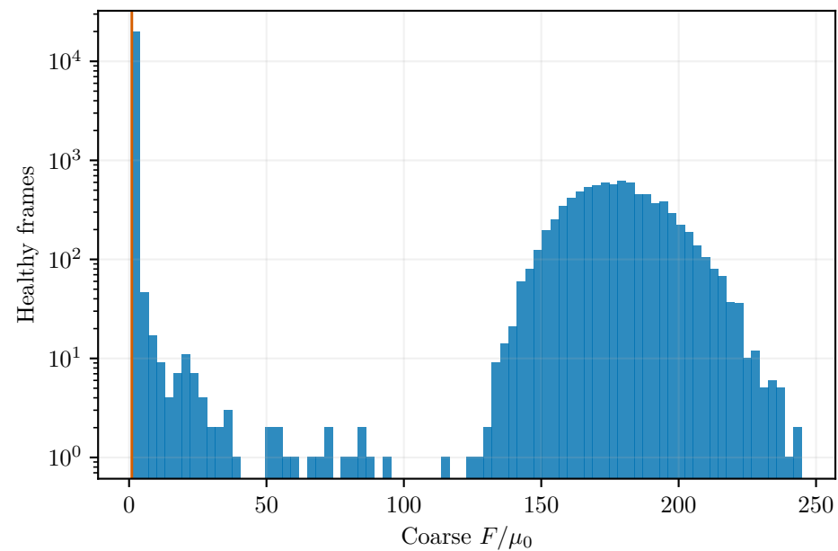
Channel 32 (frequency ID 568): health-filtered scalar distributions N=28,209; stored coarse mask rate 71.09%
