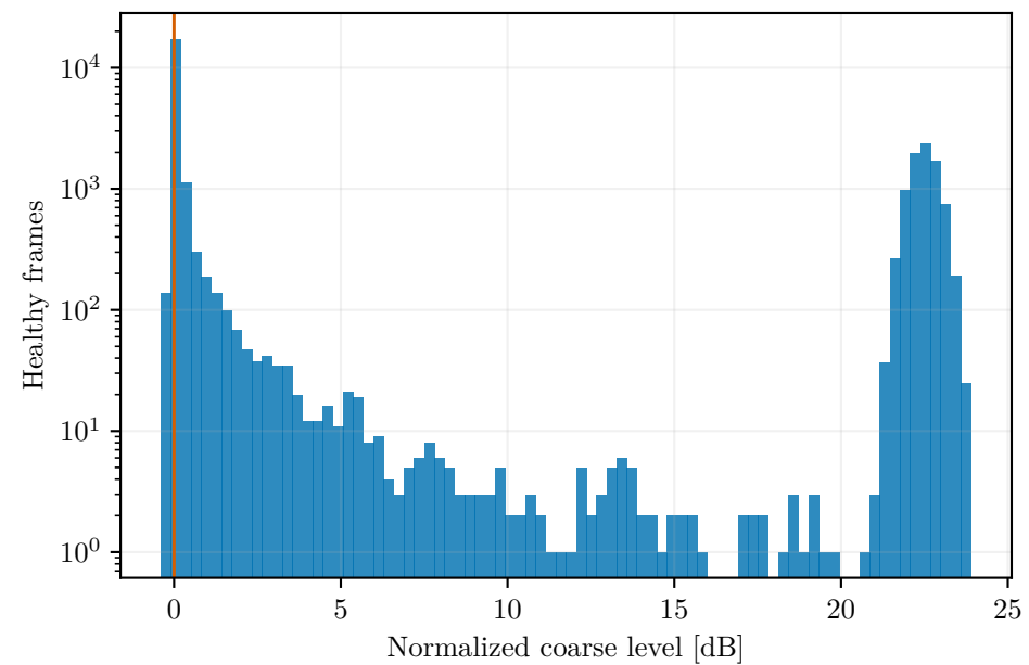
Channel 32 (frequency ID 568): health-filtered scalar distributions N=28,209; stored coarse mask rate 71.09%
