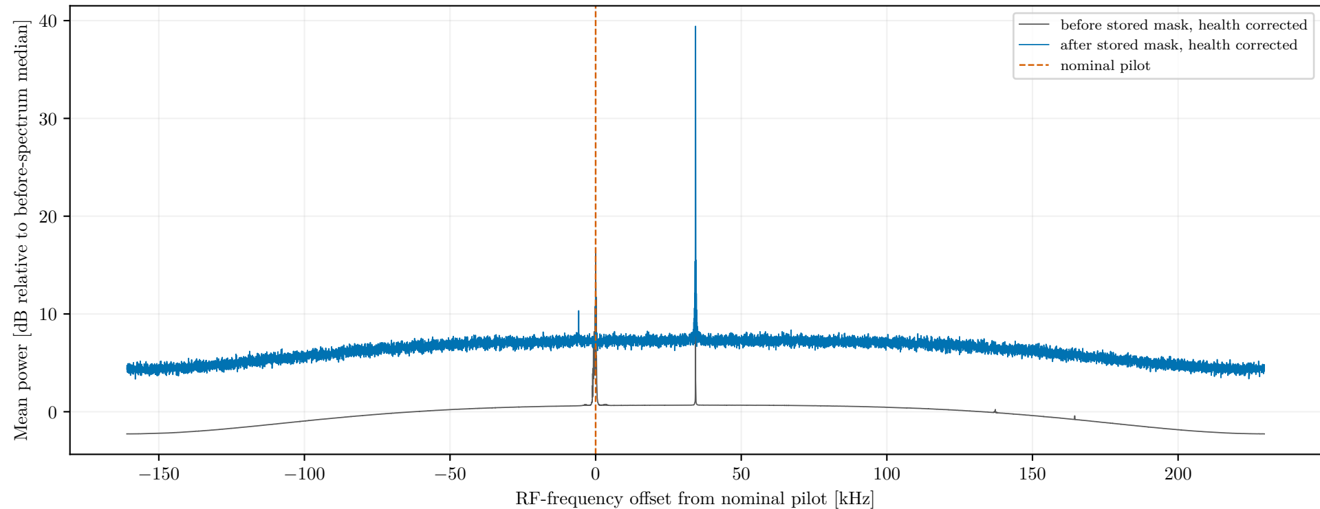
Channel 36 (frequency ID 506): relative time-averaged spectra exact v1 DC subtraction: 5 before, 5 after
