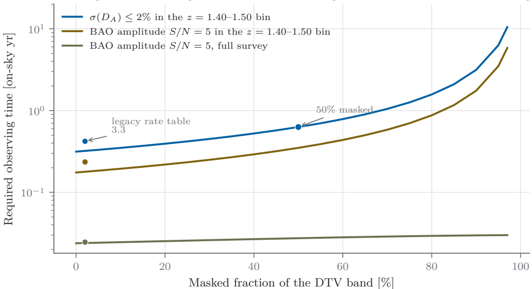
Masking cost: observing time to reach BAO targets versus uniform DTV masking
