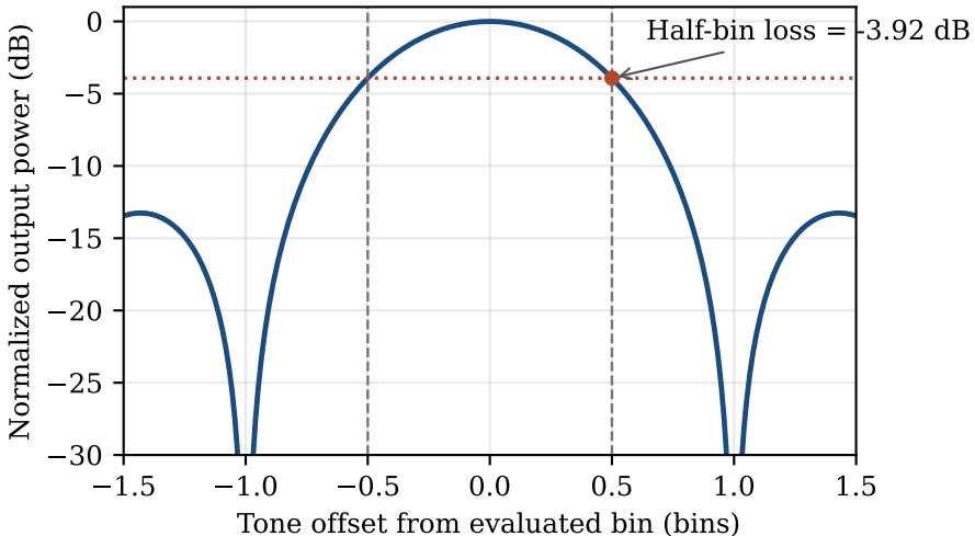
Rectangular-window single-bin mismatch ( N = 64 )
