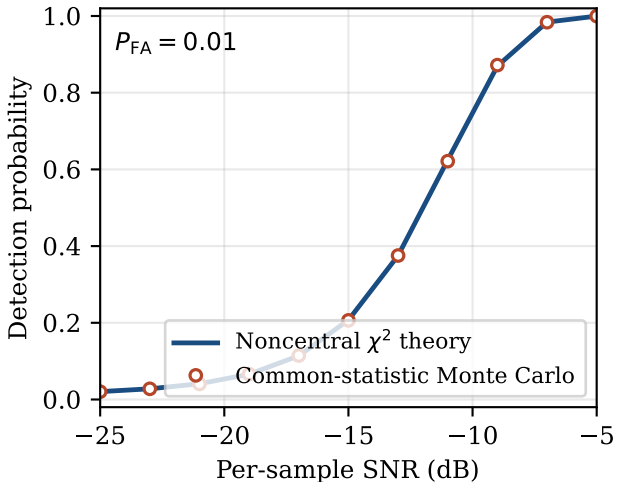
(a) Detection-probability verification ( N = 64 )
