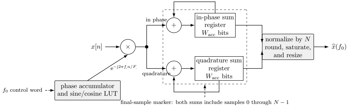
Figure 21: Selected-frequency Fourier-sum architecture. Both accumulators include the final accepted sample before normalization.
