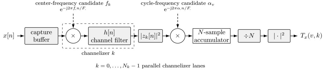
Figure 12: This buffered CAF-DFT reference realization frequency-shifts x[n] by each physical center-frequency candidate f_k and passes each shifted version through a low-pass filter, a process referred to as channelization. The magnitude squared produces the zero-lag autocorrelation sequence. Correlation with the cycle-frequency kernel at the physical candidate \alpha_v , accumulation of N samples, and division by N produce \hat{C}_x(\alpha_v, f_k) . Its magnitude squared is the nonnegative test statistic T_x(v, k) .
