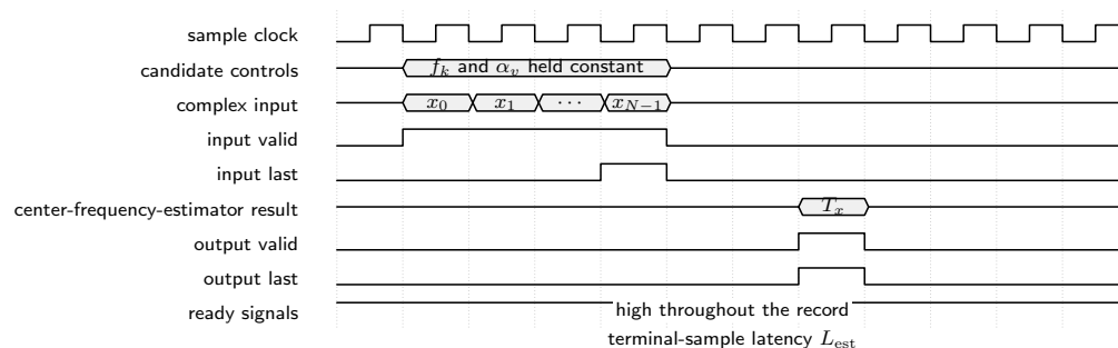
Figure 18: Symbolic continuous-rate timing of the center-frequency estimator; both control words remain fixed for each N -sample record, and one statistic is emitted after the terminal sample.
