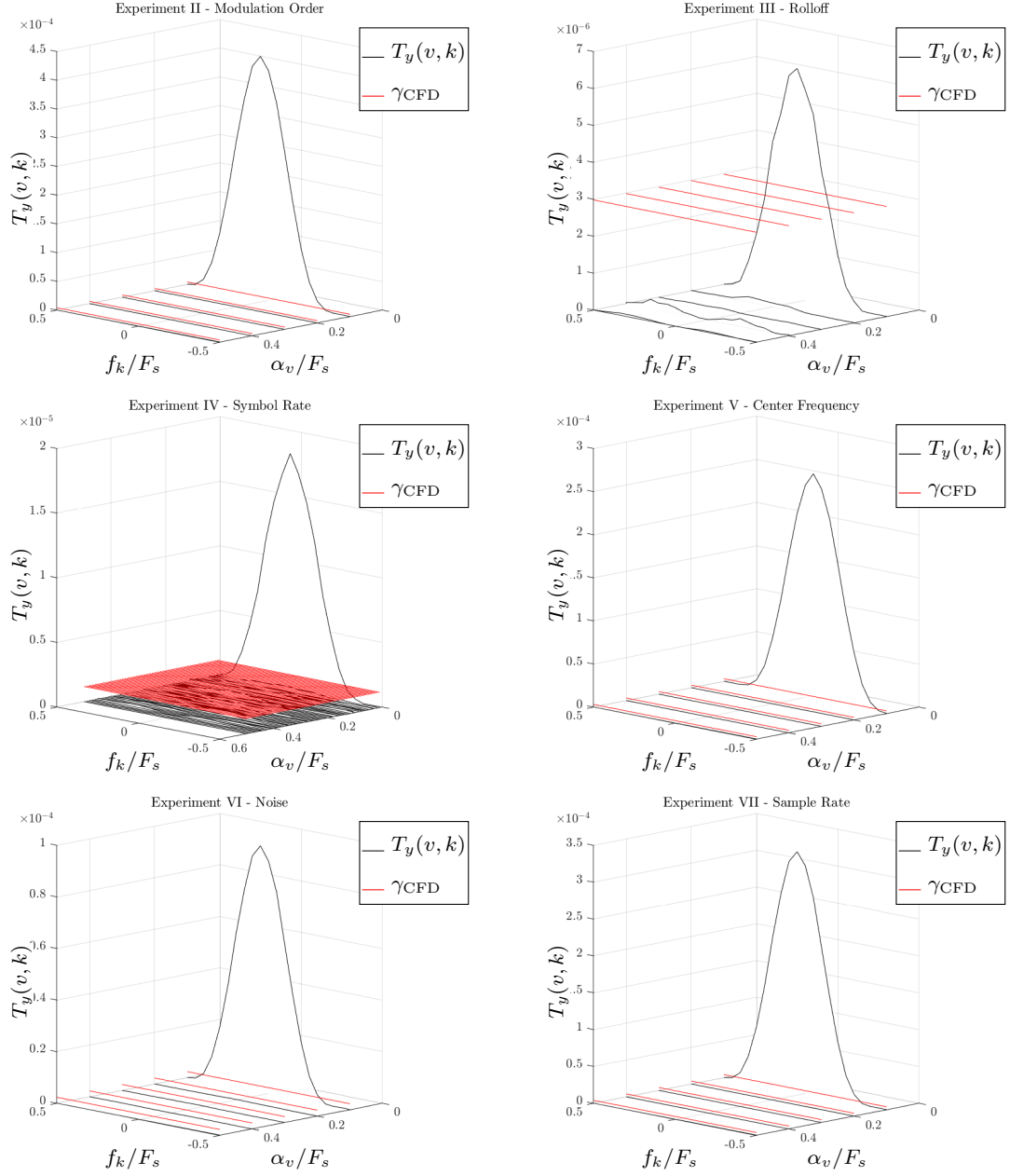
Figure 36: Streaming-SCA test-statistic plots for Experiments II–VII.
