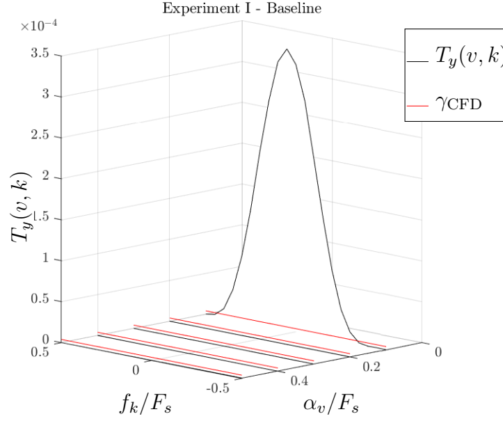
Figure 35: Streaming-SCA test-statistic plot for Experiment I.
