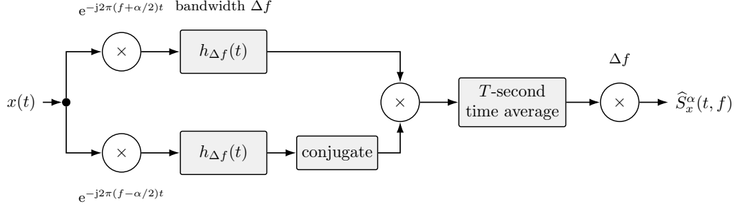
Figure 10: As described by Gardner in [3], this baseline SCA shifts the components centered at f + \alpha/2 and f - \alpha/2 to baseband. The component centers are separated by \alpha . The shifted signals pass through low-pass filters h_{\Delta f}(t) with bandwidth \Delta f and unity-passband height before their outputs are correlated, time-averaged over T , and scaled by \Delta f . The ideal SCF S_X^\alpha(f) is obtained in the ordered limits T \rightarrow \infty and then \Delta f \rightarrow 0 .
