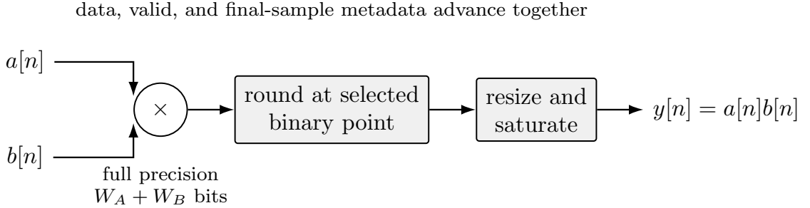
Figure 31: Fixed-point multiplier architecture with explicit rounding and saturation stages.
