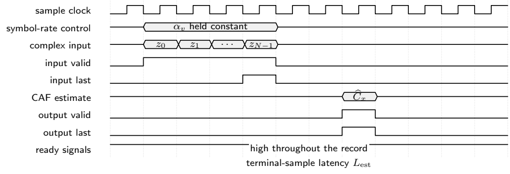
Figure 20: Symbolic continuous-rate timing of the symbol-rate estimator with an aligned terminal result, valid tag, and final-sample tag.
