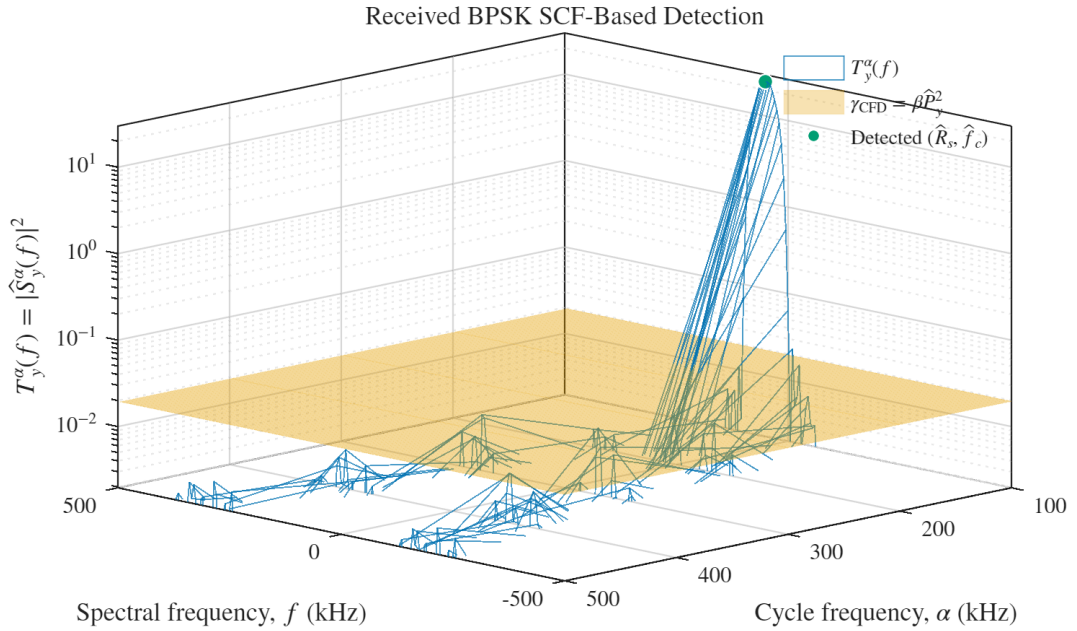
Figure 15: Full SCF test statistic for a received BPSK-SRRC waveform with R_s = 100 kBd, f_c = 50 kHz, and requested E_b/N_0 = 14 dB. The nontrivial cycle-frequency slices are compared with the flat empirical threshold \gamma_{\text{CFD}} = 10^{-2} \hat{P}_y^2 . Only the 100-kHz slice exceeds the threshold, and its maximum occurs at 50 kHz.
