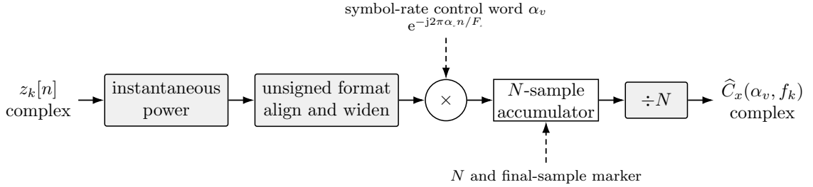
Figure 19: Functional architecture of the symbol-rate estimator, including the non-negative fixed-point format boundary after instantaneous power.
