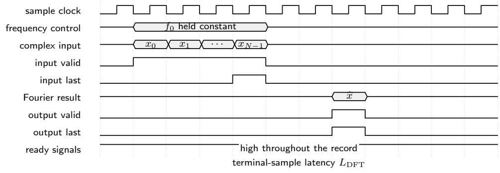
Figure 22: Symbolic continuous-rate timing of the selected-frequency Fourier-sum evaluator; the normalized Fourier result follows the terminal input sample by fixed latency.
