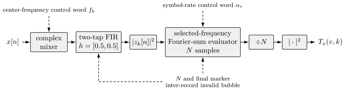
Figure 17: Functional architecture of the center-frequency estimator. Solid arrows carry sampled data; dashed arrows carry configuration and block control.
