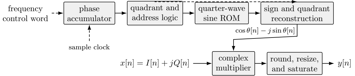
Figure 23: Functional architecture of the frequency mixer. The NCO phase advances once per sample clock during continuous-rate operation.
