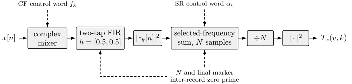
Figure 17: Functional architecture of the CFE module. Solid arrows carry sampled data; dashed arrows carry configuration and block control.
