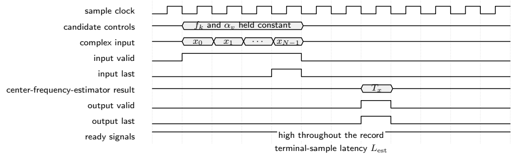
Figure 18: Symbolic continuous-rate timing of the center-frequency estimator; both control words remain fixed for each N -sample record, and one statistic is emitted after the terminal sample.
