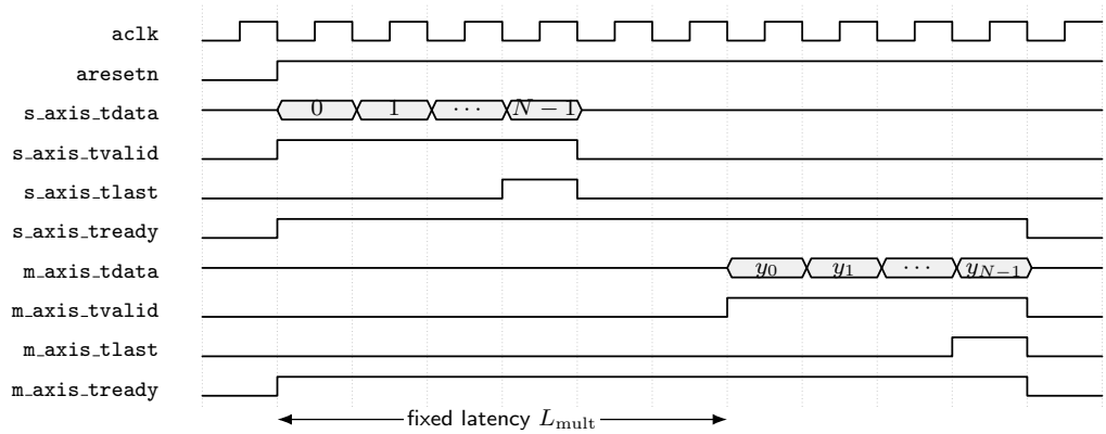
Figure 32: Symbolic AXI4-Stream timing of the fixed-point multiplier module. The product on tdata remains aligned with tvalid and tlast through stalls.
