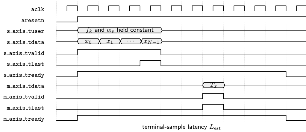
Figure 18: Symbolic AXI4-Stream timing of the center-frequency estimator; both control words remain fixed for each N -sample record, and one statistic is emitted after the terminal input transfer.
