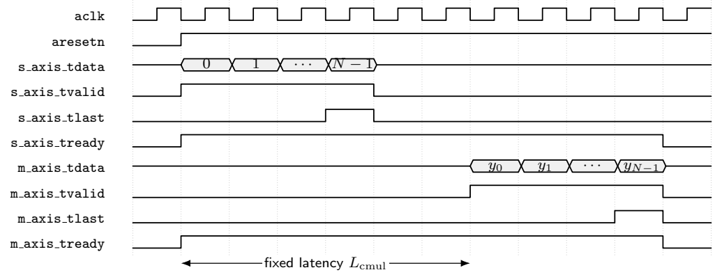
Figure 30: Symbolic AXI4-Stream timing of the complex-multiplier module. Each accepted, aligned input pair produces one complex product.
