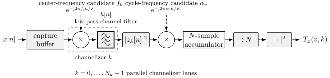
Figure 12: This buffered CAF-DFT reference realization frequency-shifts x[n] by each physical center-frequency candidate f_k and passes each shifted version through a low-pass filter, a process referred to as channelization. The magnitude squared produces the zero-lag autocorrelation sequence. Correlation with the cycle-frequency kernel at the physical candidate \alpha_v , accumulation of N samples, and division by N produce \hat{C}_x(\alpha_v, f_k) . Its magnitude squared is the nonnegative test statistic T_x(v, k) .
