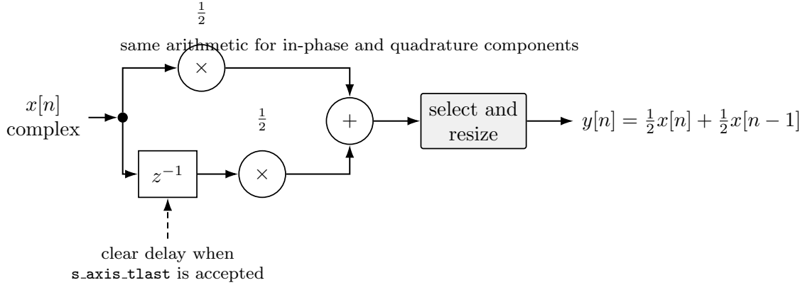
Figure 25: Configured two-tap complex low-pass filter with coefficients [0.5, 0.5] .
