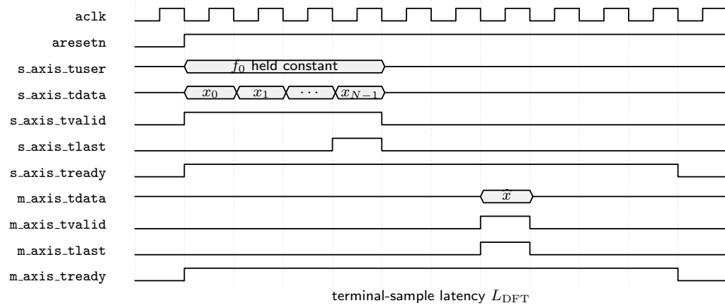
Figure 22: Symbolic AXI4-Stream timing of the selected-frequency Fourier-sum evaluator; the normalized Fourier result follows the accepted terminal input transfer.
