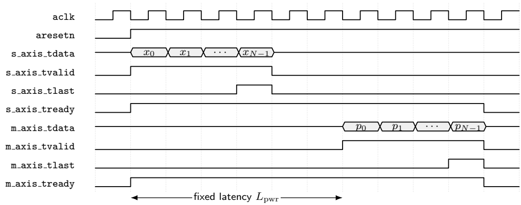
Figure 28: Symbolic AXI4-Stream timing of the instantaneous-power module. Each accepted complex input produces one nonnegative output.
