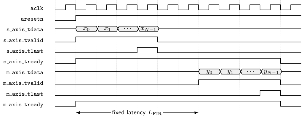
Figure 26: Symbolic AXI4-Stream timing of the two-tap low-pass filter module. The tdata , tvalid , and tlast fields remain aligned through stalls.
