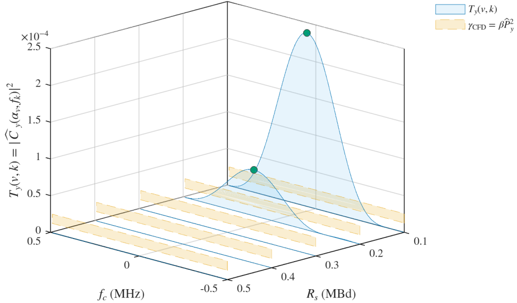
Figure 16: Streaming SCA test statistic T_y(v, k) = |\hat{C}_y(\alpha_v, f_k)|^2 for two M-QAM-SRRC signals in a shared noise floor. The transmitted parameter pairs are (R_s, f_c) = (100 \text{ kBd}, 50 \text{ kHz}) and (200 \text{ kBd}, 100 \text{ kHz}) . Both pairs lie on the estimator grid, both row maxima identify the transmitted center frequencies, and both exceed the constant threshold \gamma_{\text{CFD}} = \beta \hat{P}_y^2 with \beta = 10^{-3} . Green markers indicate the detected row maxima.
