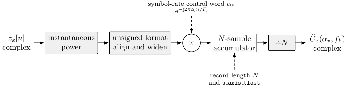
Figure 19: Functional architecture of the symbol-rate estimator, including the non-negative fixed-point format boundary after instantaneous power.
