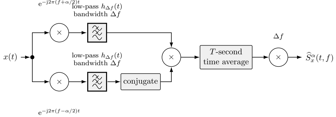
Figure 10: As described by Gardner in [3], this baseline SCA shifts the components centered at f + \alpha/2 and f - \alpha/2 to baseband. The component centers are separated by \alpha . The shifted signals pass through low-pass filters h_{\Delta f}(t) with bandwidth \Delta f and unity-passband height before their outputs are correlated, time-averaged over T , and scaled by \Delta f . The ideal SCF S_X^\alpha(f) is obtained in the ordered limits T \rightarrow \infty and then \Delta f \rightarrow 0 .
