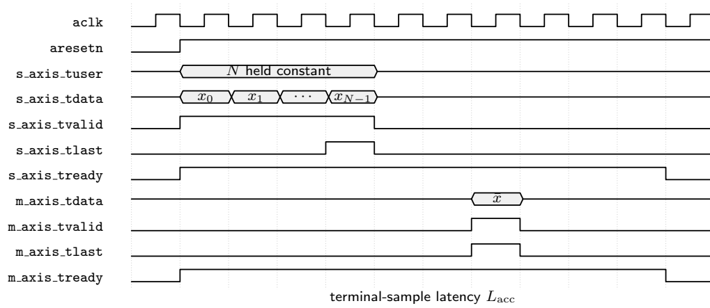
Figure 34: Symbolic block-synchronous timing of the accumulator module. The input s.axis.tlast accompanies sample N - 1 , and the output value \bar{x} = s[N - 1]/N is emitted after that sample has been included.
