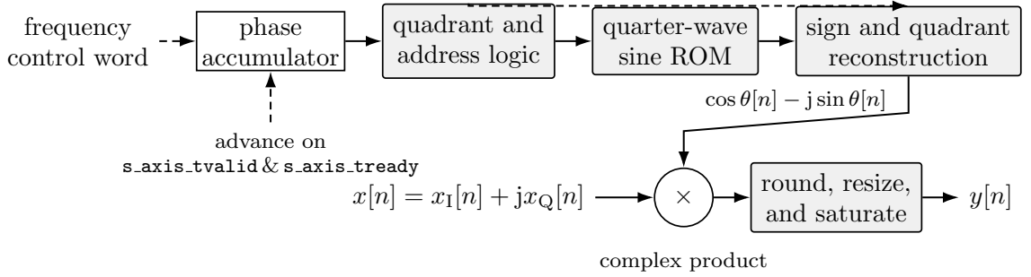
Figure 23: Functional architecture of the frequency mixer. The NCO phase advances once per accepted input transfer.
