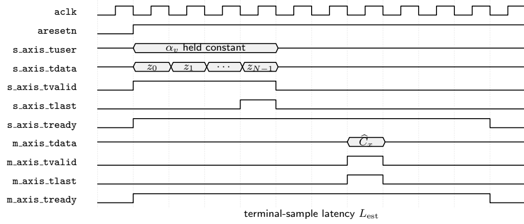
Figure 20: Symbolic AXI4-Stream timing of the symbol-rate estimator with aligned m_axis_tdata , m_axis_tvalid , and m_axis_tlast .
