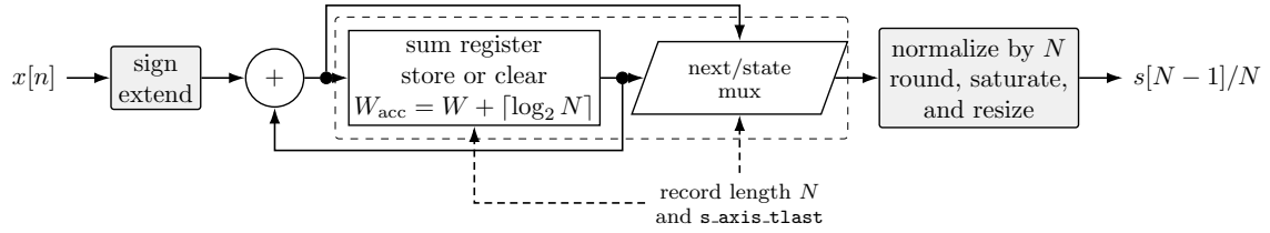
Figure 33: Block-synchronous accumulator architecture. The final accepted sample is included before the terminal sum is normalized and emitted.
