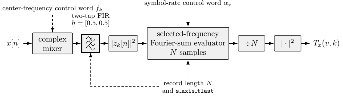
Figure 17: Functional architecture of the center-frequency estimator. Solid arrows carry sampled data; dashed arrows carry configuration and block control.
