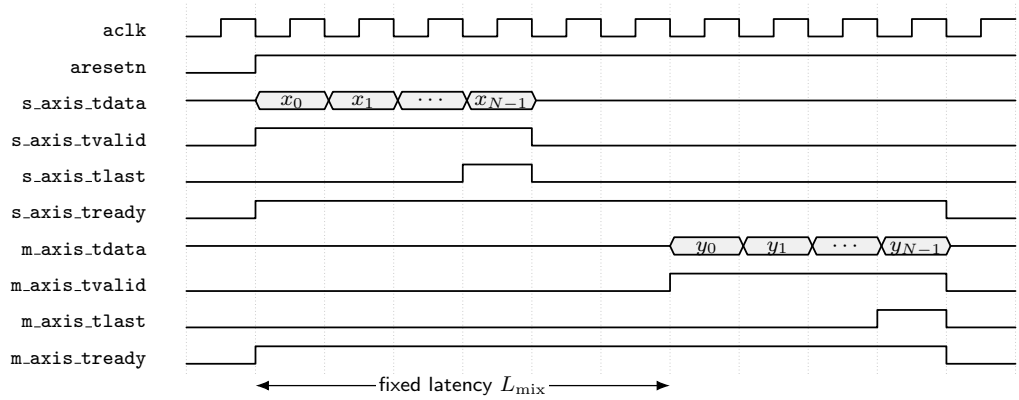
Figure 24: Symbolic AXI4-Stream timing of the frequency mixer module. The tdata , tvalid , and tlast fields remain aligned through stalls.
