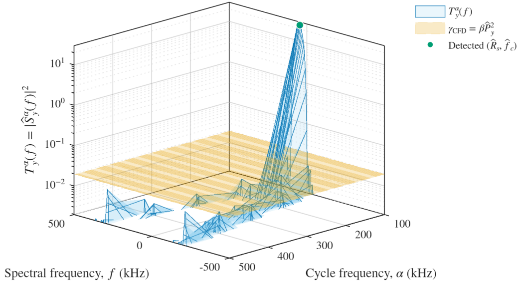
Figure 15: Full SCF test statistic for a received BPSK-SRRC waveform with R_s = 100 k Bd, f_c = 50 kHz, and requested E_b/N_0 = 14 dB. The nontrivial cycle-frequency slices are compared with the flat empirical threshold \gamma_{\text{CFD}} = 10^{-2} \hat{P}_y^2 . Only the 100-kHz slice exceeds the threshold. Its row maximum gives \hat{f}_c = 45 kHz, one 5-kHz grid bin from the transmitted center frequency.
