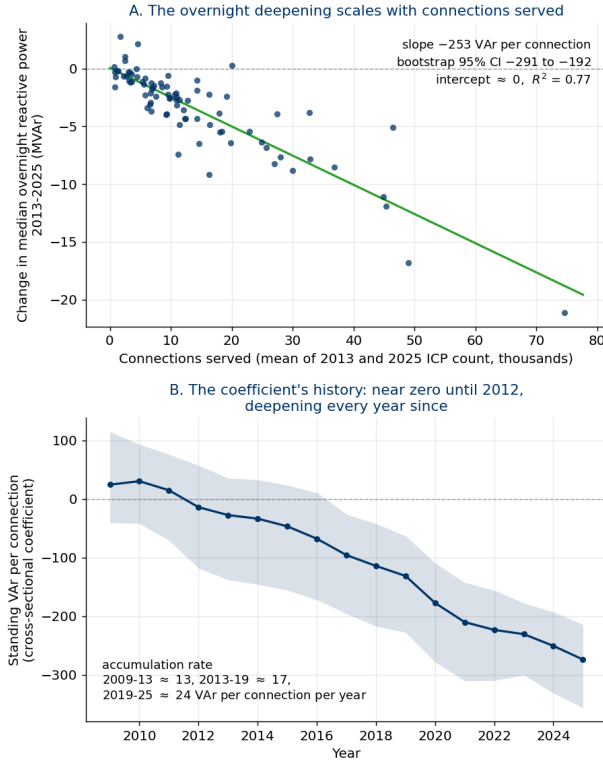
Fig. 4. The connection-scaling test. (A) Each screened grid exit point's 2013–2025 change in median overnight reactive power against the mean number of connections (ICPs) it serves ( n = 83 ): the change deepens at -253 VAr per connection (bootstrap 95% CI [-291, -192] ) with an intercept indistinguishable from zero and R^2 = 0.77 (77% of the cross-site variance explained); deleting any single grid exit point moves the slope only within [-270, -239] . Nothing about a grid-exit-point metering artefact predicts an effect proportional to the connections behind the meter. (B) The coefficient's history: the per-connection coefficient refitted across sites each year on the 81 sites present throughout 2009–2025 (shaded: bootstrap 95% CI). Near zero until 2012, it deepens every year thereafter at an accelerating rate. Sign convention: negative = added leading (capacitive) reactive power.
