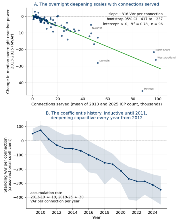
Fig. 5. The connection-scaling test. (A) Each screened panel unit's 2013–2025 change in median overnight reactive power against the mean number of connections (ICPs) it serves ( n = 96 ): the change deepens at −316 VAr per connection (bootstrap 95% CI [−417, −237]) with an intercept indistinguishable from zero and R^2 = 0.78 (78% of the cross-unit variance explained); deleting any single unit moves the slope only within [−341, −271]. Nothing about a grid-exit-point metering artefact predicts an effect proportional to the connections behind the meter. (B) The coefficient's history: the per-connection coefficient refitted across units each year on the 92 units present throughout 2009–2025 (shaded: bootstrap 95% CI). On the inductive side of zero until 2011, it crosses in 2012 and deepens every year thereafter at an accelerating rate. Sign convention: negative = added leading (capacitive) reactive power.
