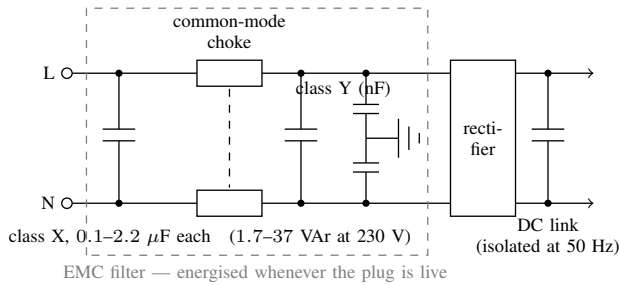
Fig. 7. The mains input stage of a switched-mode device. The EMC filter’s X-capacitance sits directly across line and neutral, ahead of the rectifier and of any standby switching, and injects \omega CV^2 of leading reactive power whenever the plug is live; the common-mode choke is transparent at 50 Hz, the Y-capacitors are nanofarad-scale, and the large DC-link capacitor is isolated from the fundamental behind the rectifier. Component values are datasheet-grade typical ranges (Section V-B).
