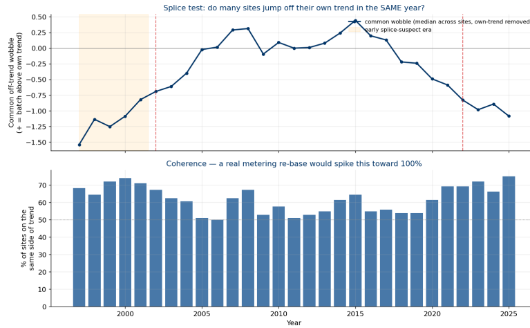
Fig. 6. Test for a system-wide metering re-base (the “splice” of the in-figure title: the join between metering eras). Each grid exit point is detrended by its own robust (Theil–Sen) line; the upper panel is the median residual across sites (the “common wobble”) and the lower panel the coherence, the share of sites on the same side of their own trend each year. A genuine re-base would spike coherence toward 100% in a single year. The change-point candidate years (about 2002 and 2022, the dashed verticals) reach only 67% and 69% against a typical-year 62%: curve-bends, not a coordinated re-base.
