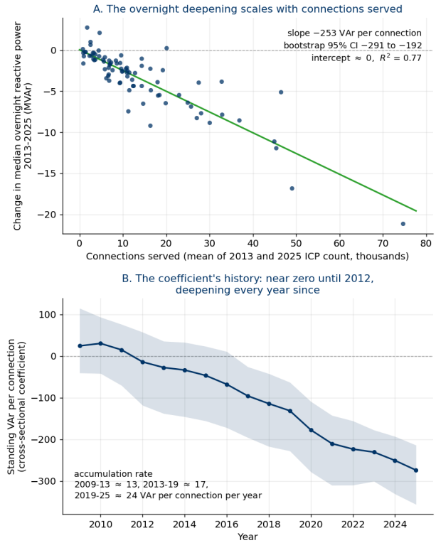
Fig. 5. The connection-scaling test. (A) Each screened grid exit point's 2013–2025 change in median overnight reactive power against the mean number of connections (ICPs) it serves ( n = 83 ): the change deepens at −253 VAr per connection (bootstrap 95% CI [−291, −192]) with an intercept indistinguishable from zero and R^2 = 0.77 (77% of the cross-site variance explained); deleting any single grid exit point moves the slope only within [−270, −239]. Nothing about a grid-exit-point metering artefact predicts an effect proportional to the connections behind the meter. (B) The coefficient's history: the per-connection coefficient refitted across sites each year on the 81 sites present throughout 2009–2025 (shaded: bootstrap 95% CI). Near zero until 2012, it deepens every year thereafter at an accelerating rate. Sign convention: negative = added leading (capacitive) reactive power.
