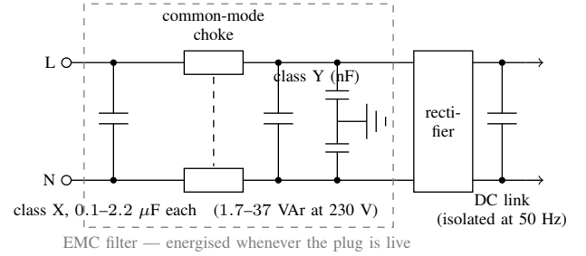
Fig. 7. The mains input stage of a switched-mode device. The EMC filter’s X-capacitance sits directly across line and neutral, ahead of the rectifier and of any standby switching, and injects \omega CV^2 of leading reactive power whenever the plug is live; the common-mode choke is transparent at 50 Hz, the Y-capacitors are nanofarad-scale, and the large DC-link capacitor is isolated from the fundamental behind the rectifier. Component values are datasheet-grade typical ranges (Section V-B).
