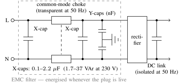
Fig. 9. The mains input stage of a switched-mode device. The EMC filter’s X-capacitance sits directly across line and neutral, ahead of the rectifier and of any standby switching, and injects \omega CV^2 of leading reactive power whenever the plug is live; the Y-capacitors are nanofarad-scale, and the large DC-link capacitor is isolated from the fundamental behind the rectifier. Component values are datasheet-grade typical ranges (Section V-B); on North America’s 120 V, 60 Hz mains the same 0.1–2.2 \mu\text{F} range injects 0.5–12 VAr.
