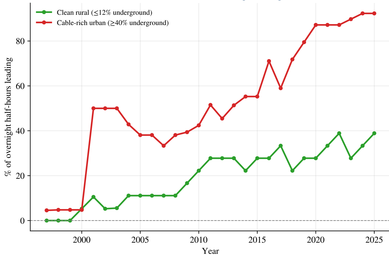
Even clean rural networks go leading
