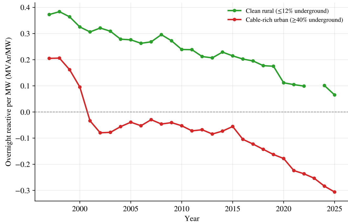
Per-MW drift: clean vs cable-rich
