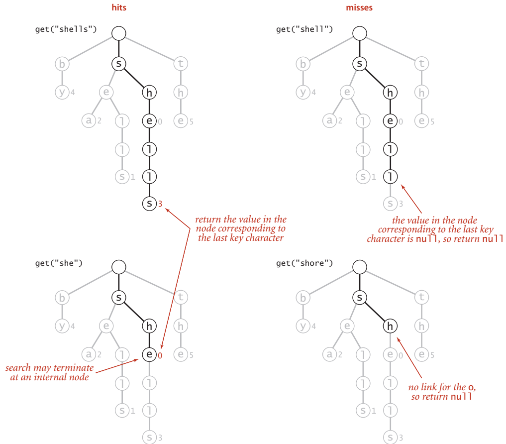
Trie search examples
