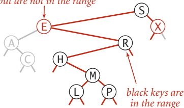
Range search in a BST
