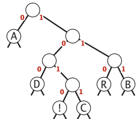
A Huffman code
