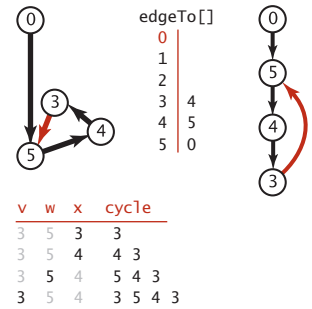
Trace of cycle computation
