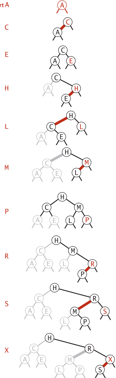
Red-black BST construction traces
