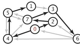
Shortest-paths data structures
