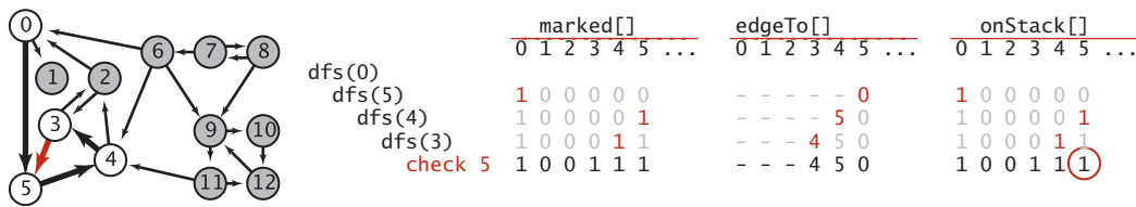
Finding a directed cycle in a digraph
