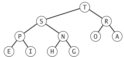
A heap-ordered complete binary tree
