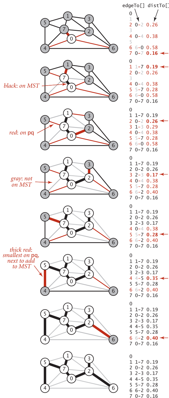
Trace of Prim's algorithm (eager version)
