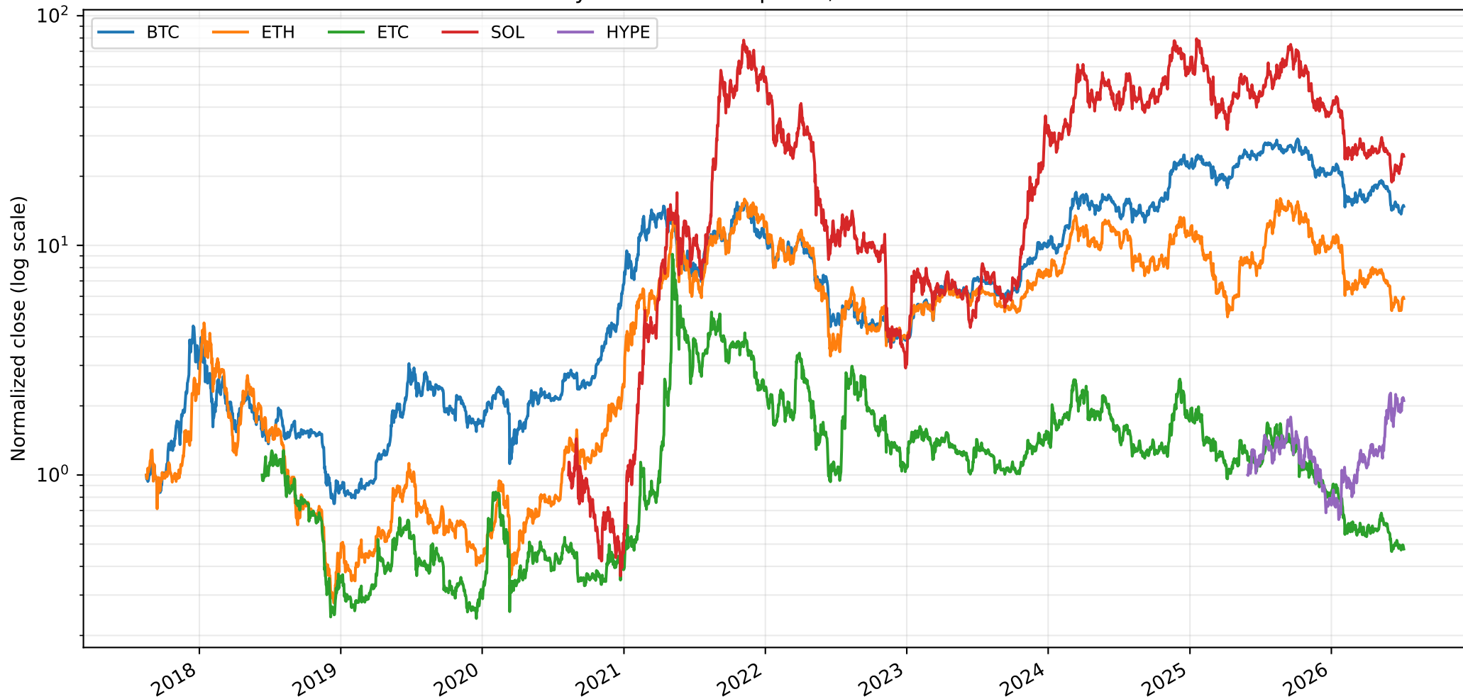
Daily Binance close prices, normalized to 1
