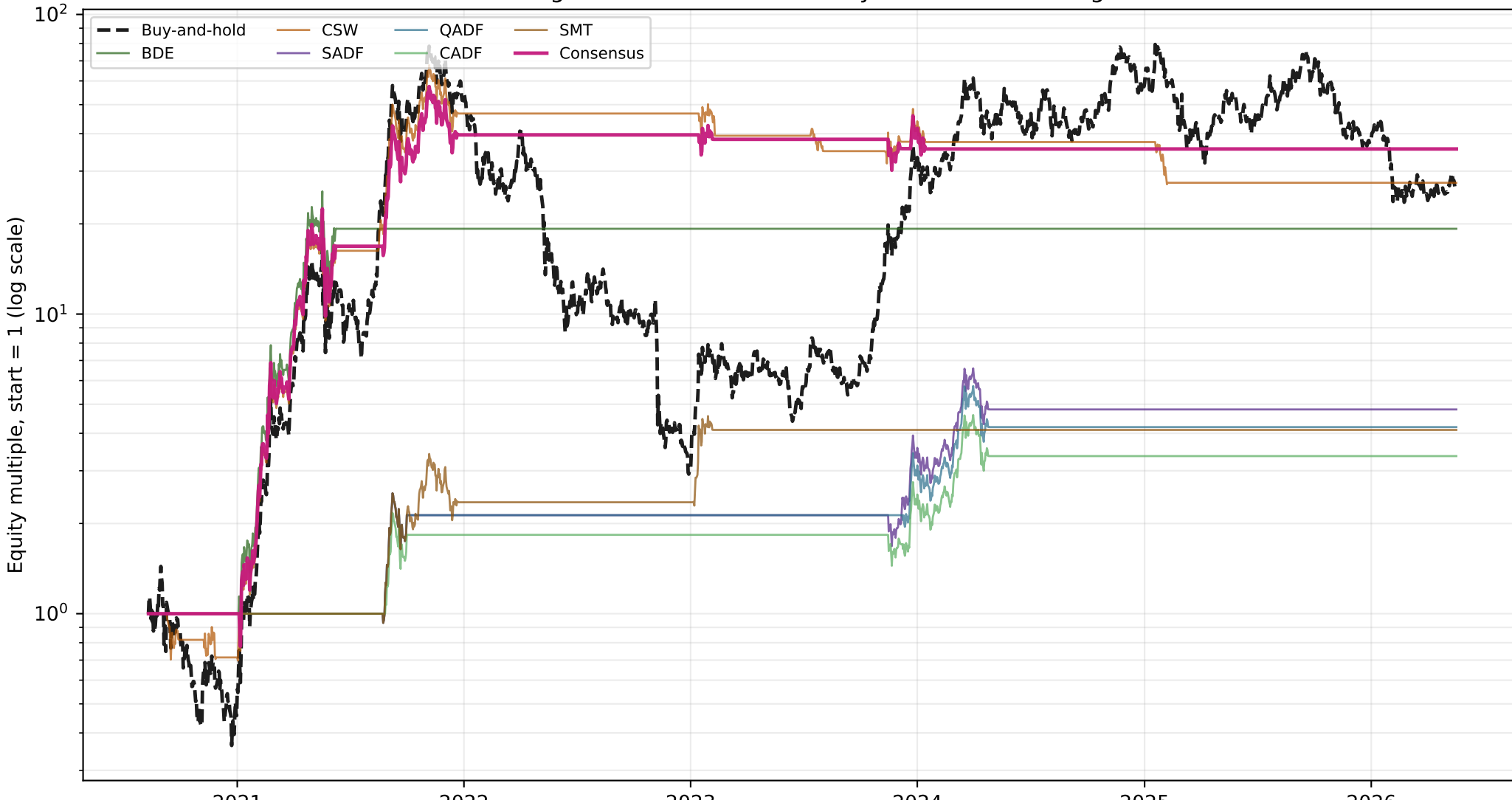
SOL: long/flat PnL curves from daily structure-break signals
