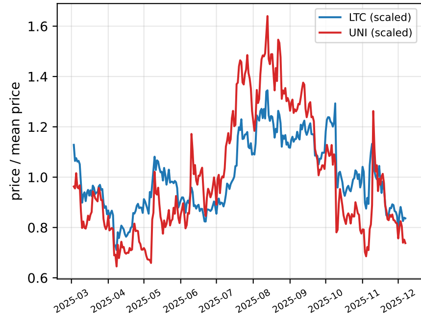
(a) Midprices relative to their mean
