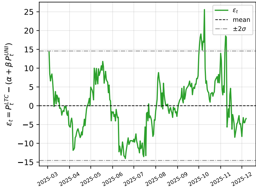
(b) Co-integration factor
