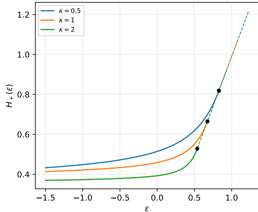
Optimal exit: value function H_+ (solid=continue, dashed=exercise, •=trigger \varepsilon^* ) (a) H_+ , varying \kappa ( \rho = 0.05 )
