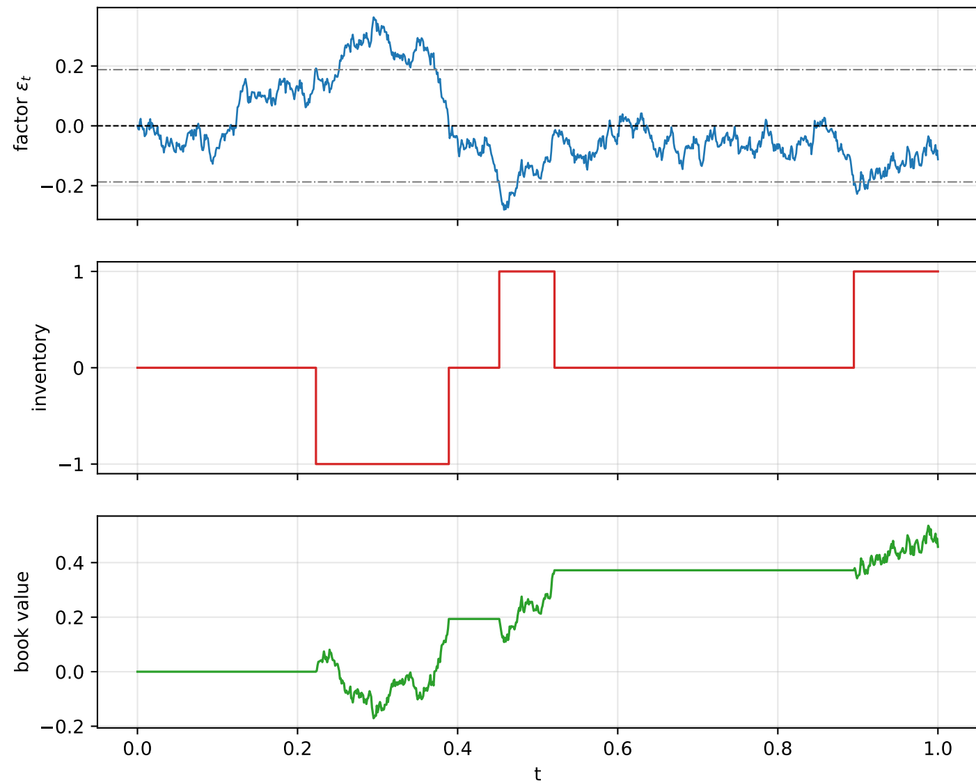
Naive band strategy (entry at \pm 1.3\sigma_{stat} , exit near the mean)
