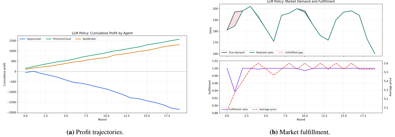
Figure 2: Round-level behavior from the repository’s LLM experiments.
