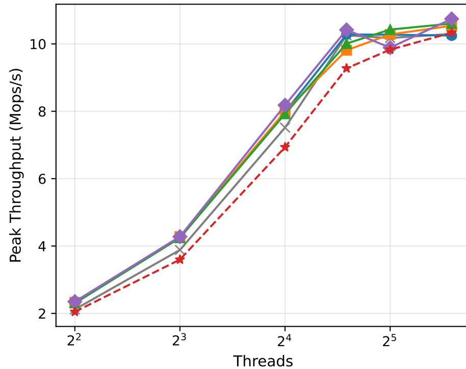
YCSB D (95% R / 5% I)
