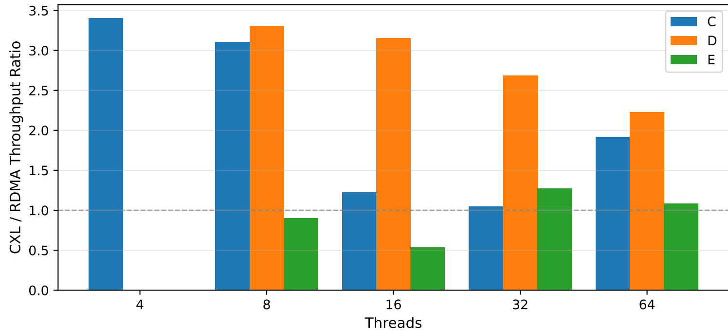
CXL Throughput Speedup vs RDMA per Workload
