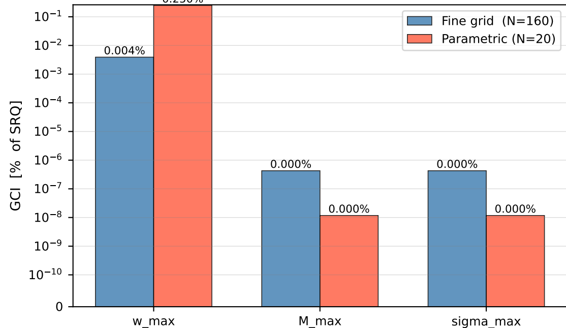
Discretization Uncertainty (GCI): Fine Grid (N=160) vs. Parametric Grid (N=20)
