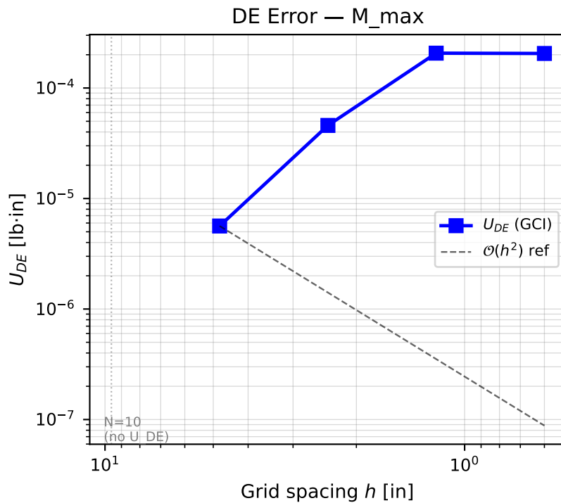
Discretization Error U_{DE} vs. Grid Spacing h 8-ft LVL Header, q_0 = 500 lb/ft
