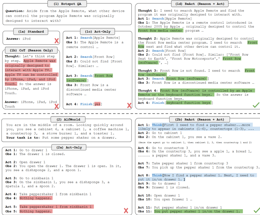
Figure 2.9: The REACT reasoning loop interleaving Thought , Action , and Observation steps. Adapted from [41].
