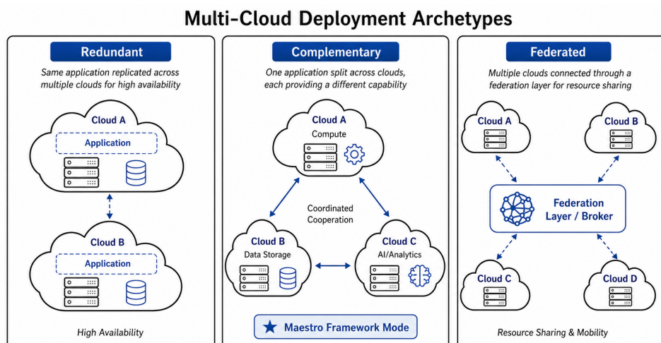
Figure 2.12: Multi-cloud deployment archetypes - redundant, complementary, and federated strategies - as classified by Petcu [28]. The Maestro framework operates in complementary mode.
