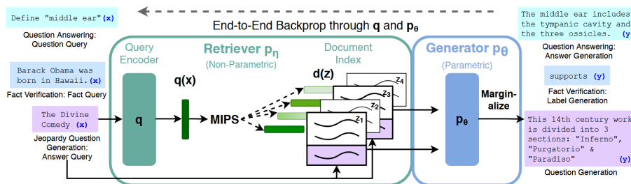
Figure 2.5: End-to-end RAG architecture combining a DPR retriever with a BART-large generator. Adapted from [21].
