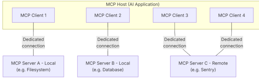
Figure 2.5: Model Context Protocol architecture showing the Host, Client, and Server roles connected via JSON-RPC 2.0. Adapted from [28].
