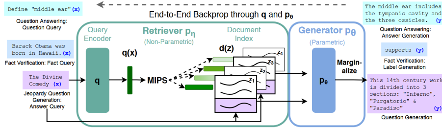
Figure 2.2: End-to-end RAG architecture combining a DPR retriever with a BART-large generator. Adapted from [22].
