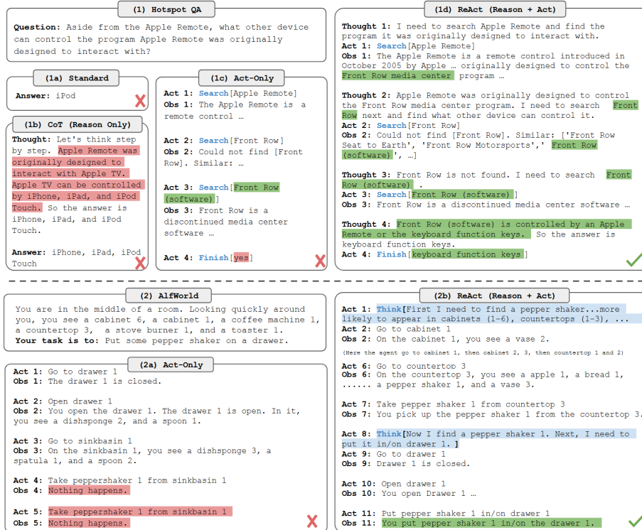
Figure 2.9: The REACT reasoning loop interleaving Thought , Action , and Observation steps. Adapted from [35].
