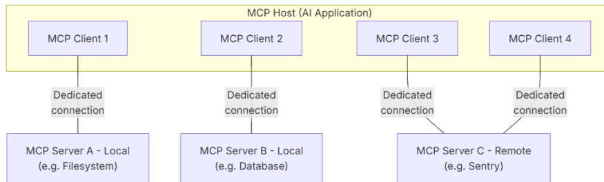
Figure 2.10: Model Context Protocol architecture showing the Host, Client, and Server roles connected via JSON-RPC 2.0. Adapted from [22].
