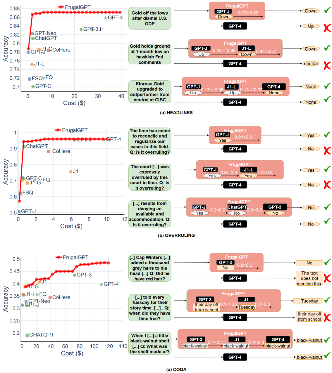
Figure 2.16: Accuracy and cost tradeoff achieved by FrugalGPT, showing that adaptive LLM cascades can reduce inference cost while maintaining or improving task performance. Adapted from Chen et al. [8].
