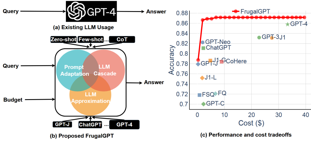
Figure 2.14: Overview of cost-reduction strategies in FrugalGPT, including prompt adaptation, LLM approximation, and LLM cascade. Adapted from Chen et al. [8].
