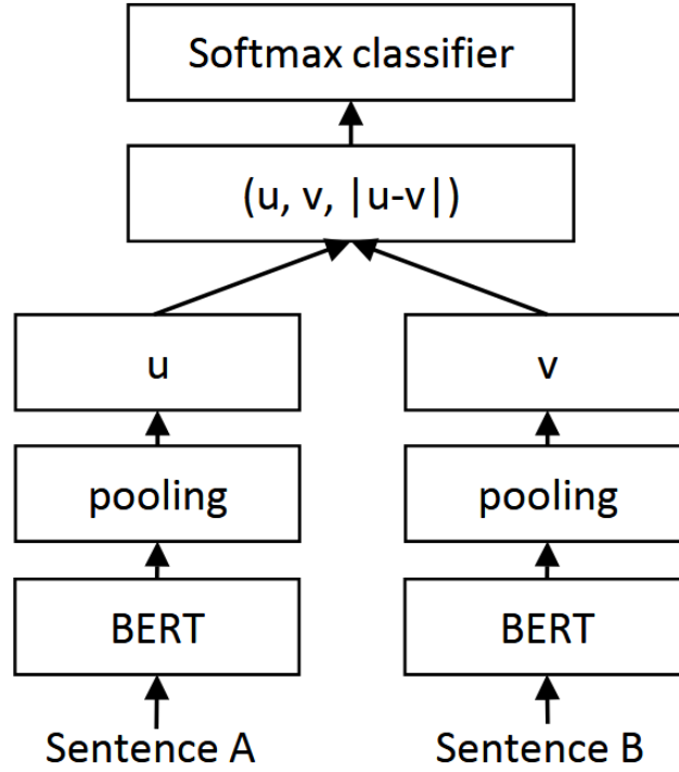
Figure 2.8: Classification and regression training objectives of SBERT. Adapted from [17].
