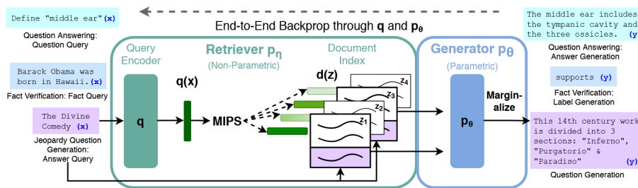
Figure 2.5: End-to-end RAG architecture combining a DPR retriever with a BART-large generator. Adapted from [19].
