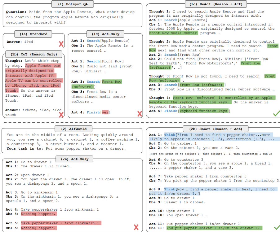
Figure 2.9: The REACT reasoning loop interleaving Thought , Action , and Observation steps. Adapted from [37].
