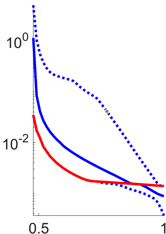
Leverett J-function
