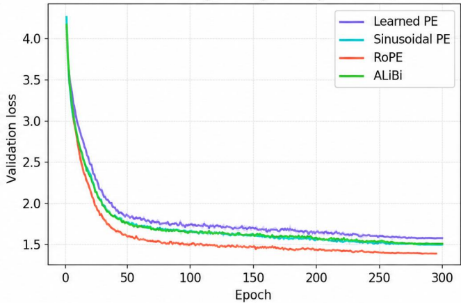
Validation loss during training — ImageNet-100 (ViT-Base)
