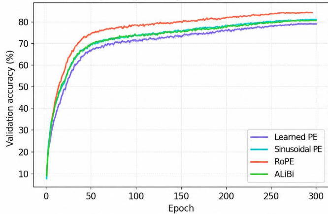
Accuracy during training — ImageNet-100 (ViT-Base)
