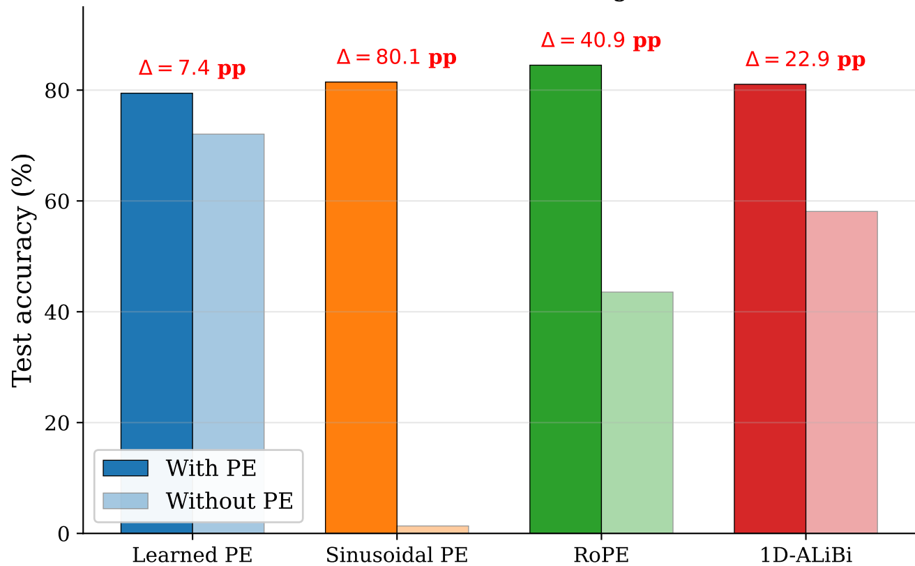
Effect of PE removal — ImageNet-100
