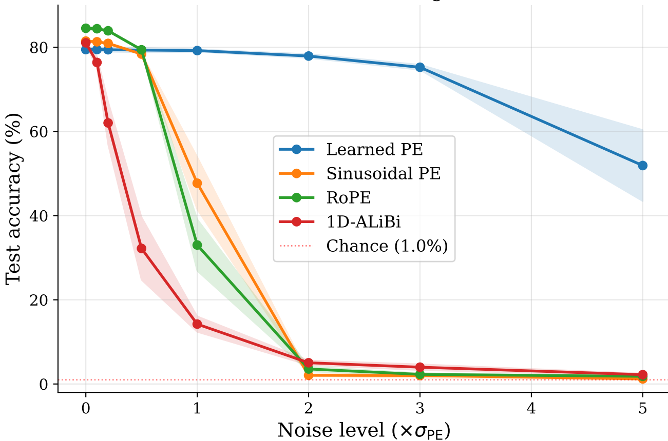
Noise robustness — ImageNet-100
