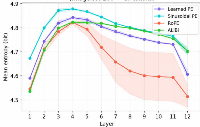
Activation entropy across layers (ImageNet-100 — all tokens)
