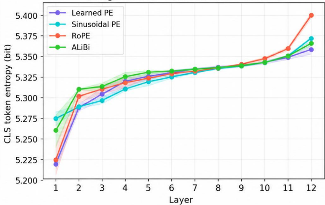
CLS token entropy across layers (ImageNet-100 — information bottleneck)
