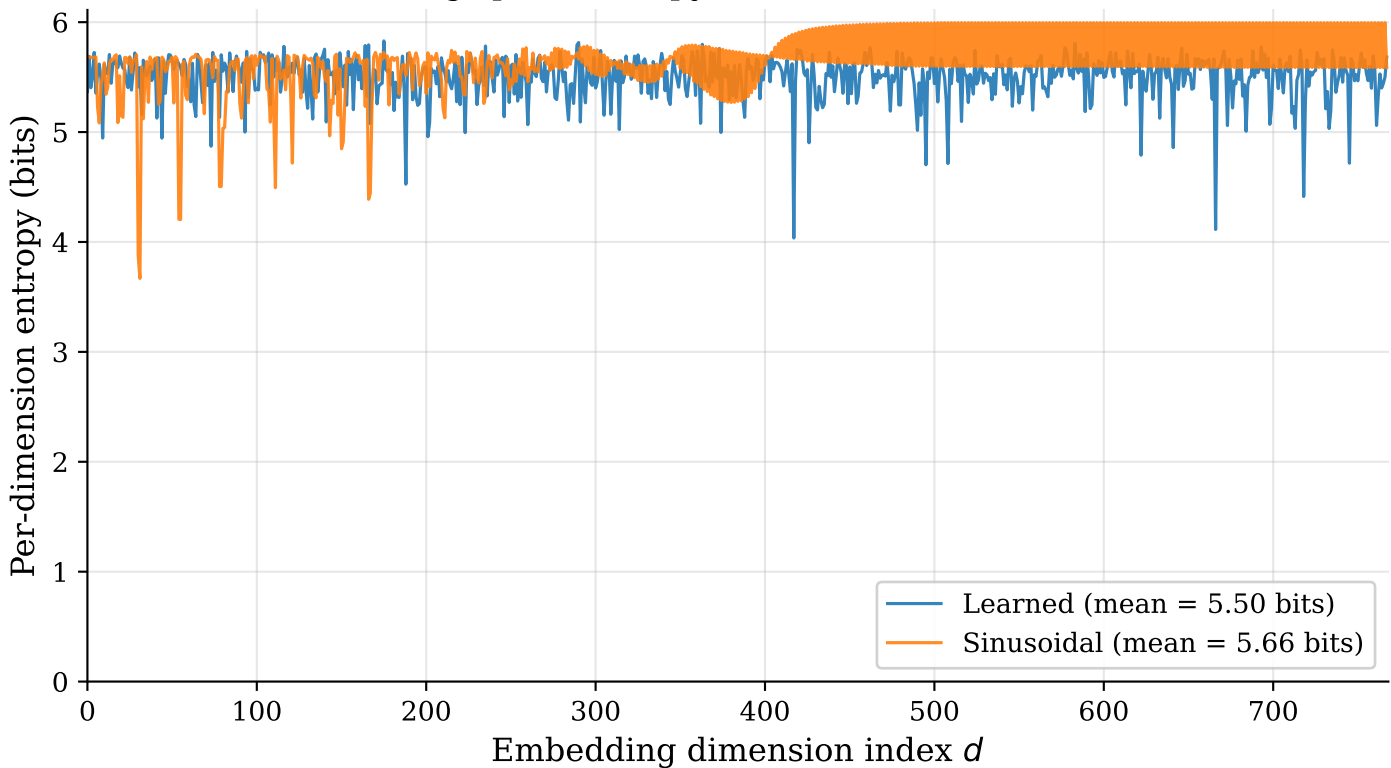
Embedding-space Entropy Profile (additive PE methods)
