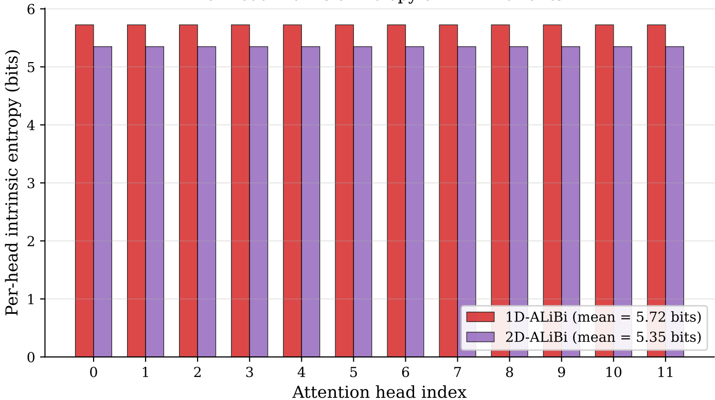
Per-head Intrinsic Entropy of ALiBi Variants
