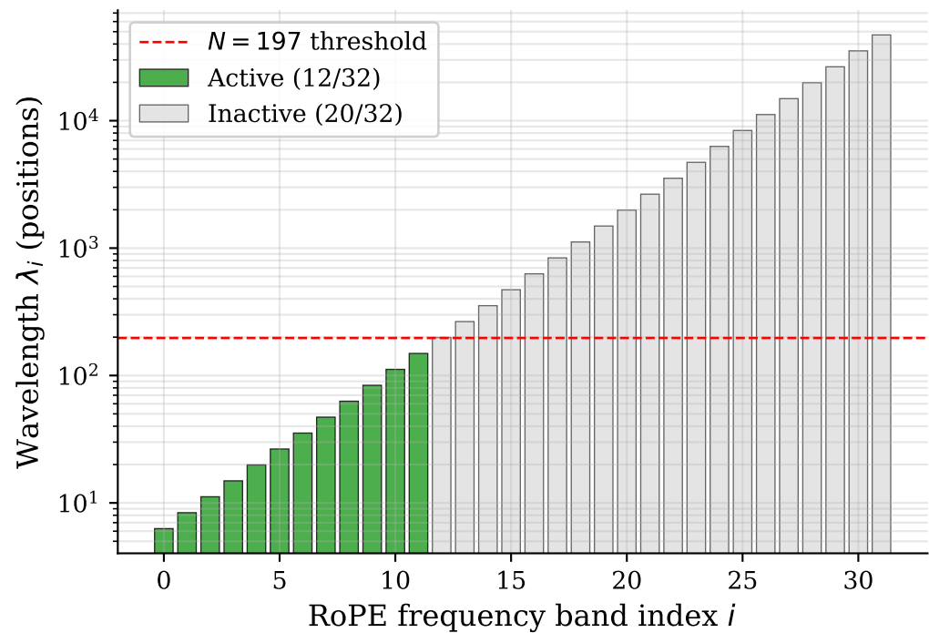
(b) RoPE rotation wavelengths (head dim d_h = 64 )
