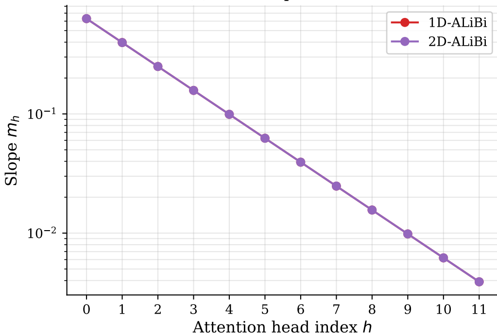
(a) ALiBi slope schedule
