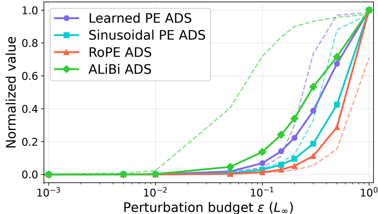
ImageNet-100 solid=ADS, dashed=accuracy loss
