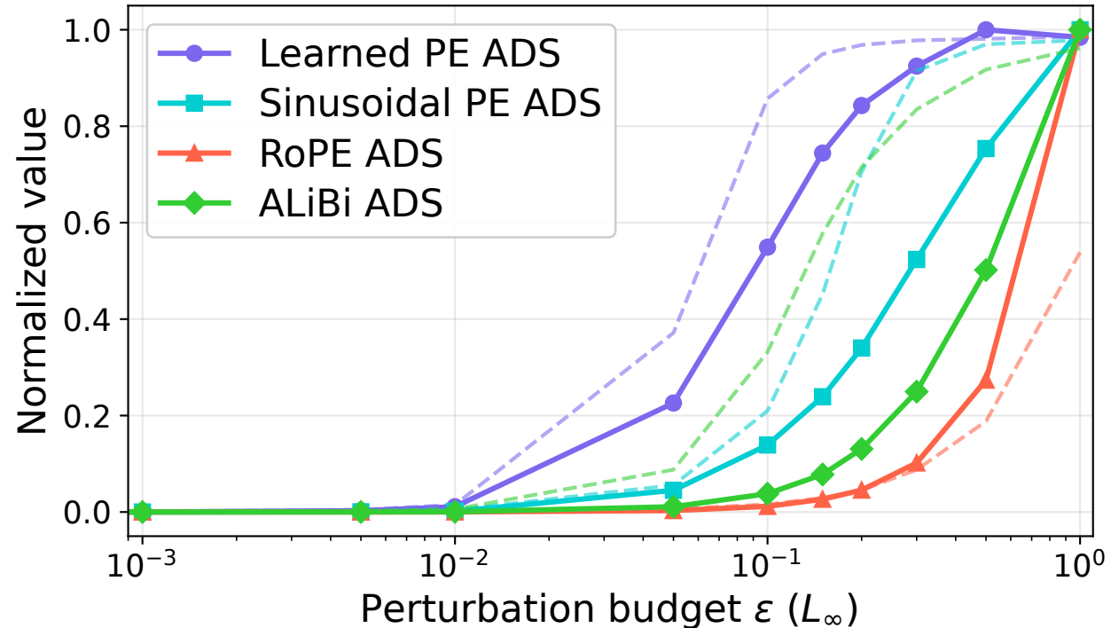
CIFAR-100 solid=ADS, dashed=accuracy loss
