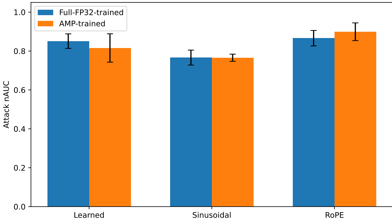
Support-matched attack nAUC ( \rho_{\max} = 0.0792384 )
