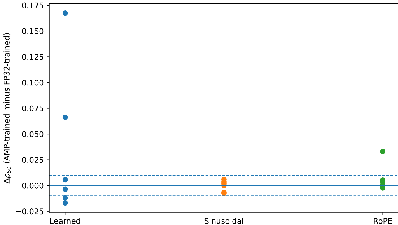
ViT-S/16 seed-matched rho50 contrasts
