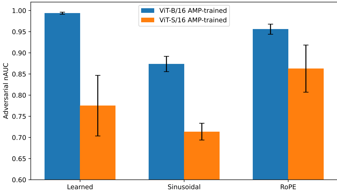
AMP-matched cross-architecture comparison ( \rho_{\max} = 0.08735 )
