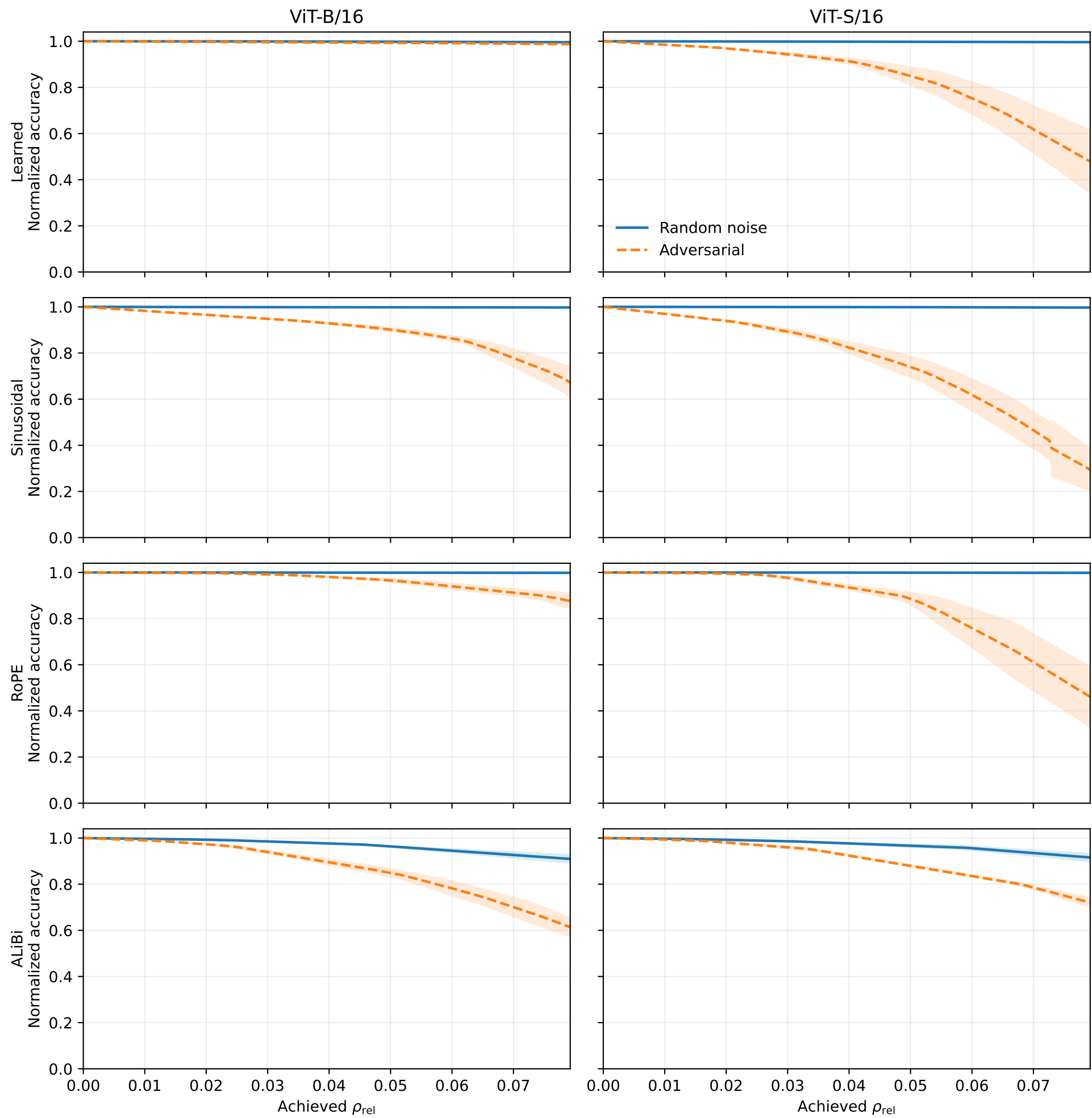
ImageNet-100 cross-architecture robustness on common support [0, 0.07924]
