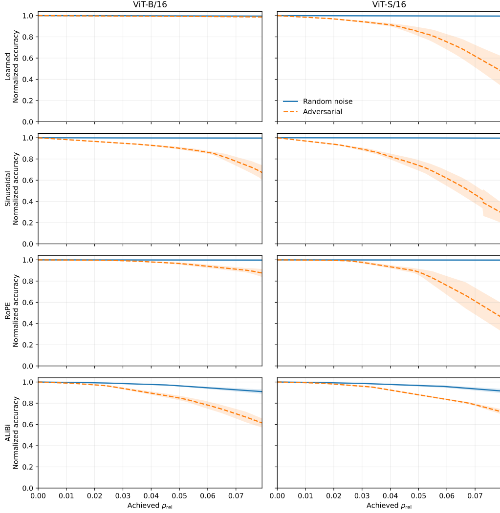
Figure 2: ImageNet-100 canonical robustness curves over the architecture-common support. Lines show across-seed means and shaded regions show \pm 1 sample SD. Random noise is solid and task-loss adversarial perturbation is dashed. Every curve is constructed at seed level before aggregation and uses the prespecified canonical native-budget grid. Post-lock all-restart audit points and direct-displacement points are not included.
