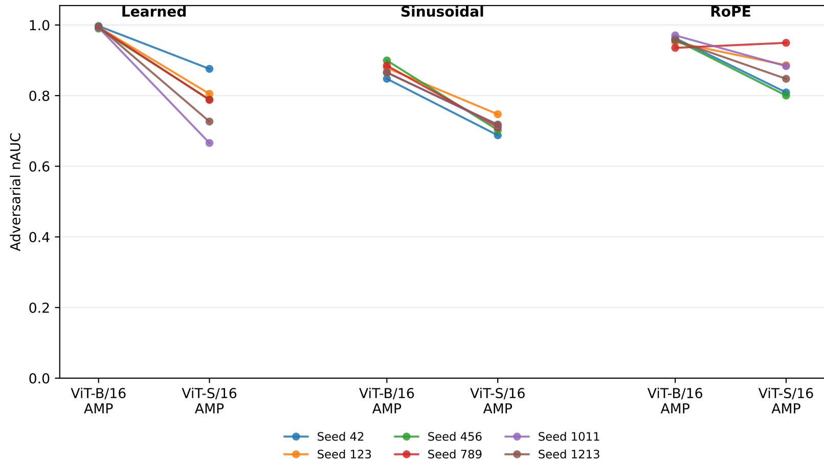
AMP-matched cross-architecture seed trajectories ( \rho_{\max} = 0.08735 )
