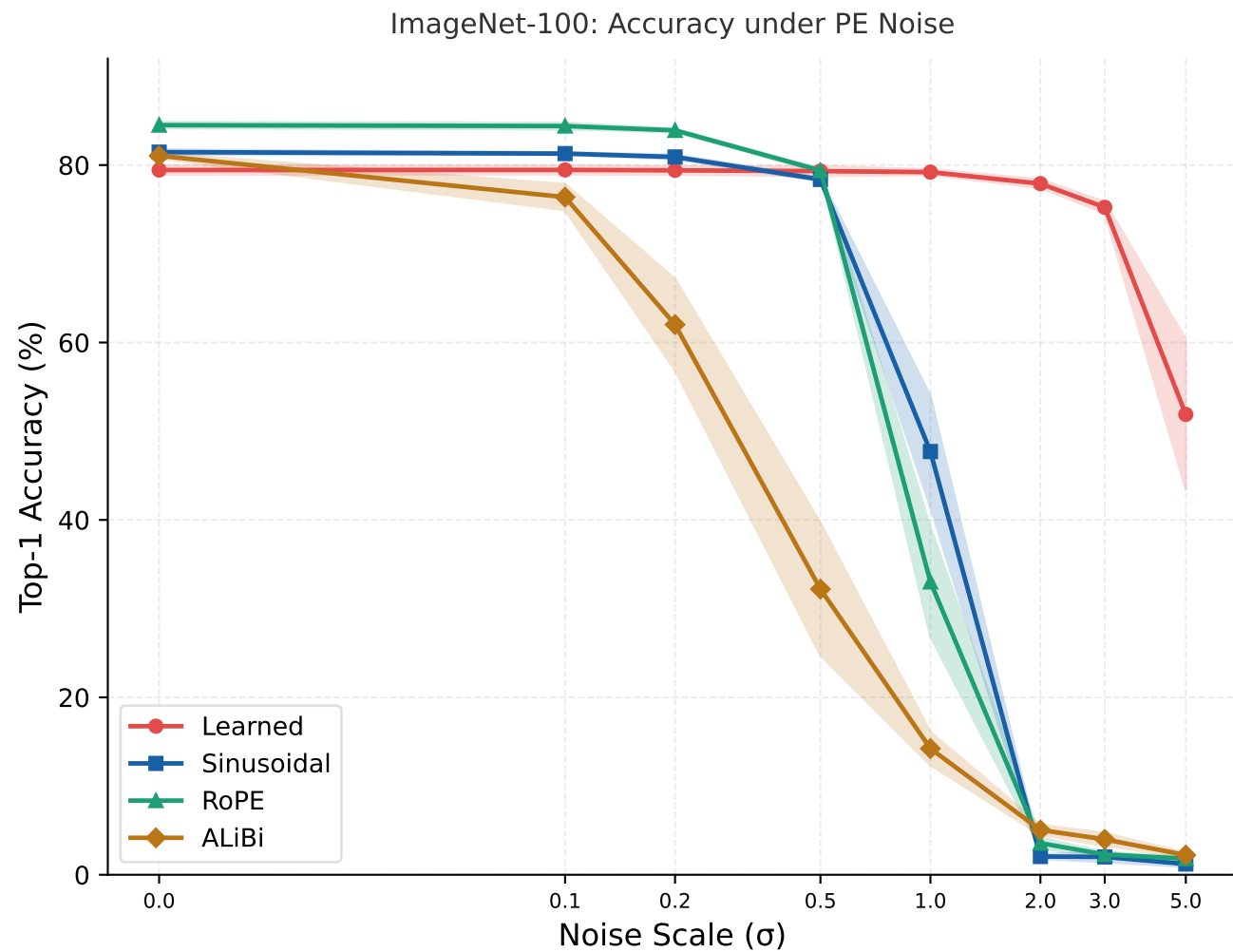
Figure 5: Noise Ablation Study — PE Robustness Gaussian noise added to positional encodings at test time (shaded = \pm\sigma , 3 seeds)
