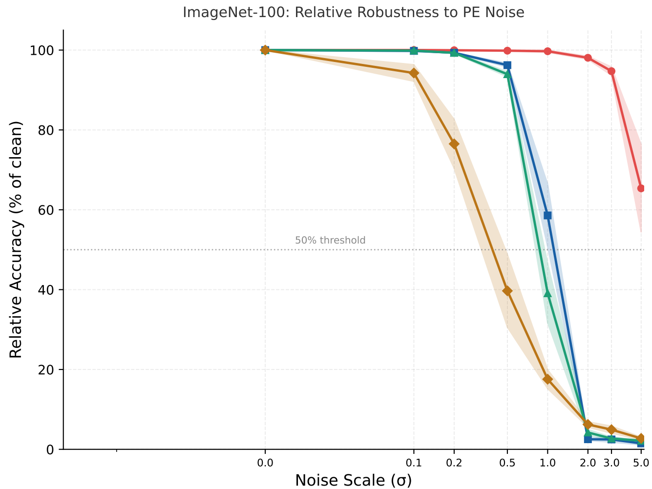
Figure 5: Noise Ablation Study — PE Robustness Gaussian noise added to positional encodings at test time (shaded = \pm\sigma , 3 seeds)
