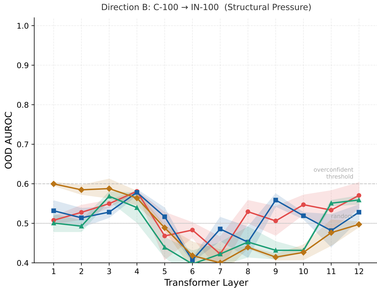
Figure 6: Layer-wise OOD AUROC — Attention Entropy as Uncertainty Score Cross-domain evaluation: in-distribution vs. OOD samples (shaded = \pm\sigma , 3 seeds)
