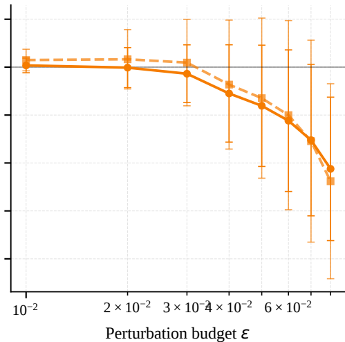
(b) CIFAR-100
