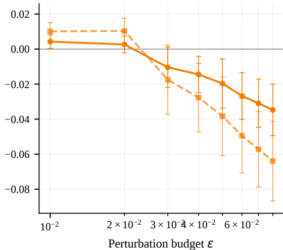
(a) ImageNet-100
